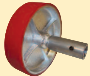
DRIVE WHEEL WITH KEYWAY & SET SCREW
