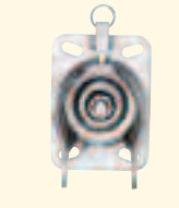
SL 4-Position Swivel Lock plunger engages at 90° angles
