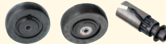
Payflex Soft Rubber non-marking tread Broncushion 60 duro. gray rubber WS Wheel Seals locks out foreign matter
