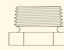
055 Pipe Tapered Thread Thread: 3/4 NPT, 1 NPT (National Pipe Thread, Nominal Dimen.) See page 69.
